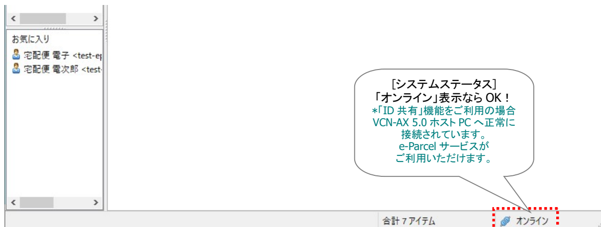
[VCN-CommCenter 画面]
